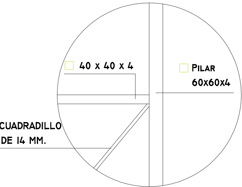
detalle 2. e_1.100
